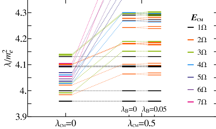
Figure 1: Using Lagrange multiplier method to lift the CM excitations. The calculation is performed in the Fock sectors |e^+e^- \rangle and |e^+e^-\gamma \rangle with M_j = 0 , \mathcal{K} = \mathcal{N}_{\max} = 8 , \sqrt{P^+\Omega} = 0.3m_e (See Section 4 for details). The vertical axis shows the eigenvalues of the light-cone Hamiltonian H_{LC} . States with different E_{CM} are colored differently. We show spectra with the lowest 50 states for three cases: \lambda_{CM} = 0 , \lambda_B = 0 ; \lambda_{CM} = 0.5 , \lambda_B = 0 and \lambda_{CM} = 0.5 , \lambda_B = 0.05 . In the last case, degeneracies caused by CM excitations are lifted.
