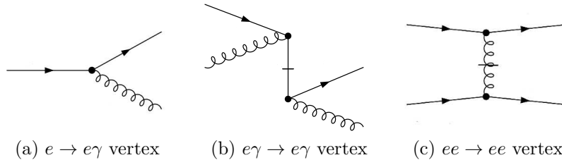
Figure 2: The relevant light-front QED vertices for positronium in the Fock sectors |e^- e^+\rangle and |e^- e^+ \gamma\rangle .
