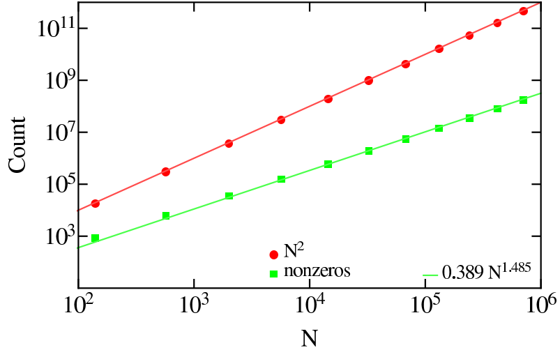
Figure 3: The sparsity of the light-cone Hamiltonian matrix H_{LC}^{(\text{pos})} . The horizontal axis is the dimensionality N of the basis space. The square dots show the number of nonzero matrix elements. A power-law fitting suggests the number of nonzero elements is proportional to \sim N^{1.485} .
