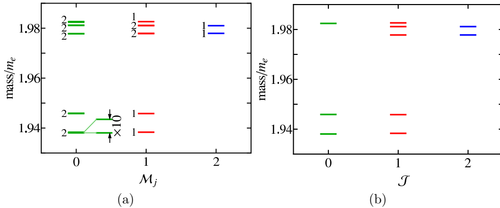
Figure 4: The positronium spectrum for (a) spin projection \mathcal{M}_j = 0, 1, 2 ; (b) total spin \mathcal{J} = 0, 1, 2 , \mathcal{M}_j = 0 identified from plot (a). For \mathcal{M}_j = 3 , there is no state within the range of the plot. The numbers to the left of the bars in plot (a) label the multiplicity of the states around each bar. Plot (a) also shows the fine splitting between the lowest \mathcal{J} = 0, \mathcal{M}_j = 0 and \mathcal{J} = 1, \mathcal{M}_j = 0 states. The total spin \mathcal{J} in plot (b) is obtained by counting the approximate degeneracy of states with different \mathcal{M}_j .
