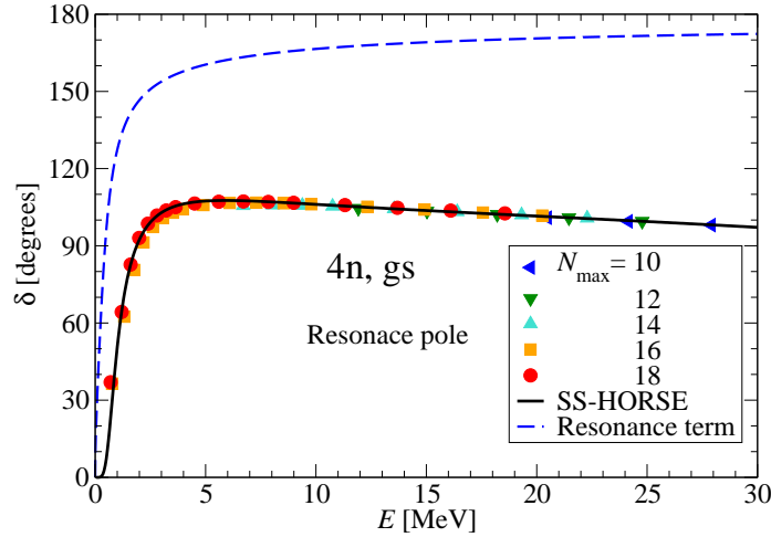
Figure 3: The 4 \rightarrow 4 scattering phase shifts: parametrization with a single resonance pole (solid line) and obtained directly from the selected NCSM results using Eq. (2) (symbols). The dashed line shows the contribution of the resonance term.
