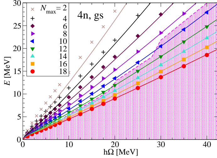
Figure 1: NCSM results for the tetraneutron ground state energy obtained with various N_{\max} (symbols) plotted as functions of \hbar\Omega . The shaded area shows the NCSM result selection for the S -matrix parametrization; the solid curves are obtained from the phase shifts parametrized with a single resonance pole by solving Eq. (2) for the eigenenergies at given N_{\max} and \hbar\Omega values.
