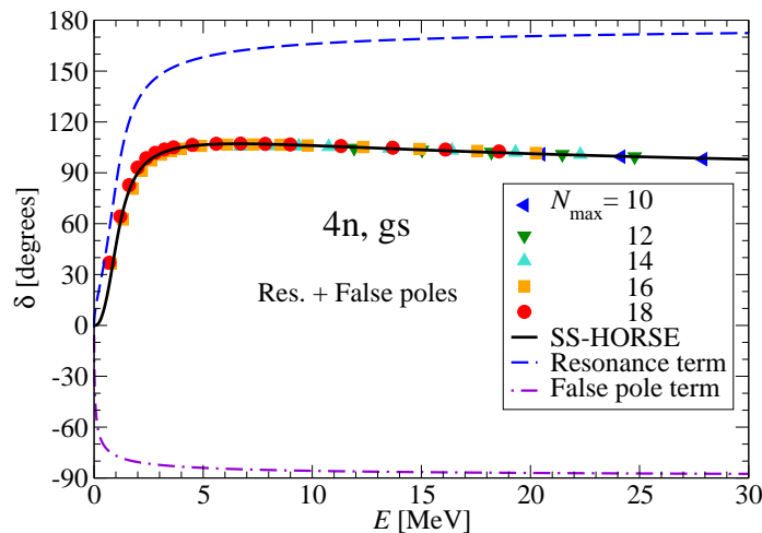
Figure 4: Same as Fig. 3 but for the parametrization with resonance and false state poles. The dashed-dotted line shows the contribution of the false state pole term.
