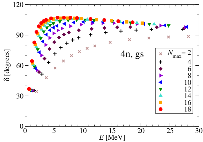
Figure 2: The 4 \rightarrow 4 phase shifts obtained directly from the NCSM results using Eq. (2).
